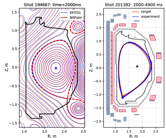
Fig. 1. DIII-D validation of NSFsim (left: flux surfaces vs EFIT) enabled RL control of plasma shape and position: agents trained in an NSFsim environment and transferred to the DIII-D PCS ran successfully in over 30 shots (right: target red, experiment blue). Clark et al., Fusion Eng. Des. (2025); Subbotin et al., Nucl. Fusion (2026).
