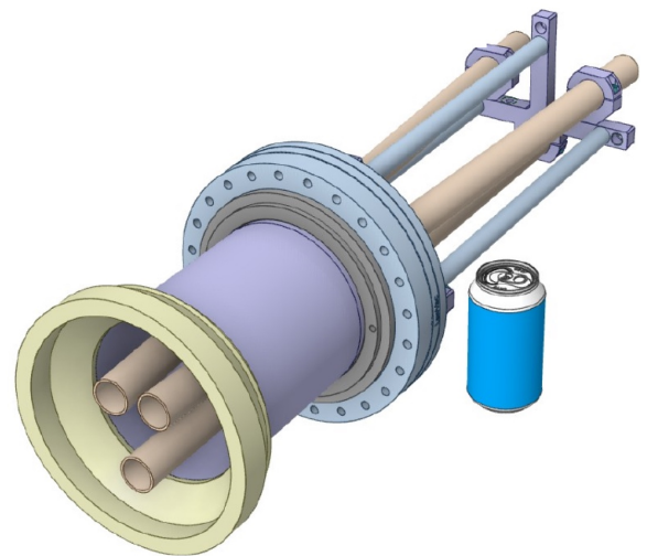
Fig. 1. MDP demonstrator for TCV, in-vessel and ex-vessel parts (CAD): an electron cyclotron emission radiometer and a profile reflectometer in one port-plug unit. It has passed its DIII-D physics validation review and is being assembled in Luxembourg. Plasma tests on TCV and DIII-D are planned for 2027.
